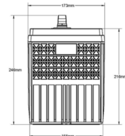
ODX-AGM31A LEFT POSITIVE SAE TERMINALS
