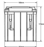
ODS-AGM70 RIGHT POSITIVE FEMALE TERMINALS
