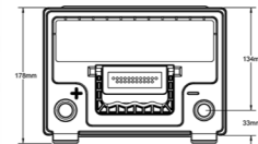
ODP-AGM75/86 LEFT POSITIVE DUAL TERMINALS (SAE & SIDE)
