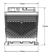
ODP-AGM48/H6/L3 RIGHT POSITIVE SAE TERMINALS
