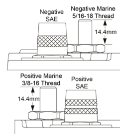
ODP-AGM34M LEFT POSITIVE DUAL TERMINALS (SAE & STUD)
