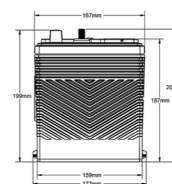
ODP-AGM34M LEFT POSITIVE DUAL TERMINALS (SAE & STUD)
